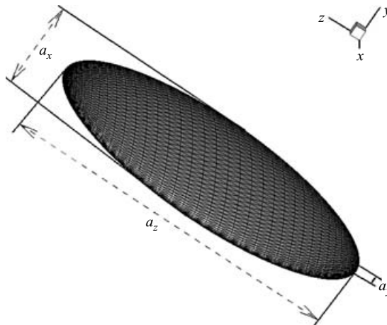
FIGURE 3. Typical ellipsoidal foil used in the current study. The surface of the ellipsoid is represented by an unstructured grid made of triangular elements.
